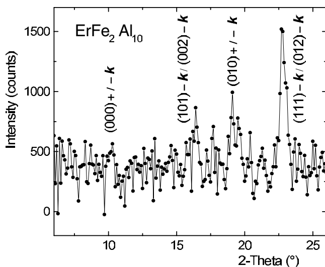
Figure 6. Difference pattern of ErFe 2 Al 10 obtained from the powder diffraction patterns at 100 mK and 3 K.
