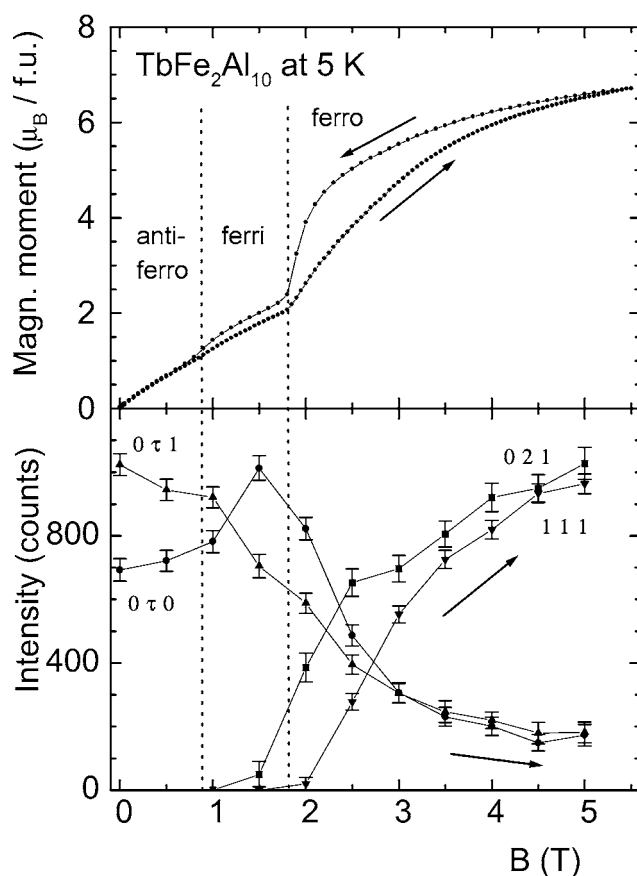
Figure 2. Field dependence of the terbium magnetic moment (upper panel) and the corresponding intensities of magnetic reflections of TbFe 2 Al 10 (lower panel).
